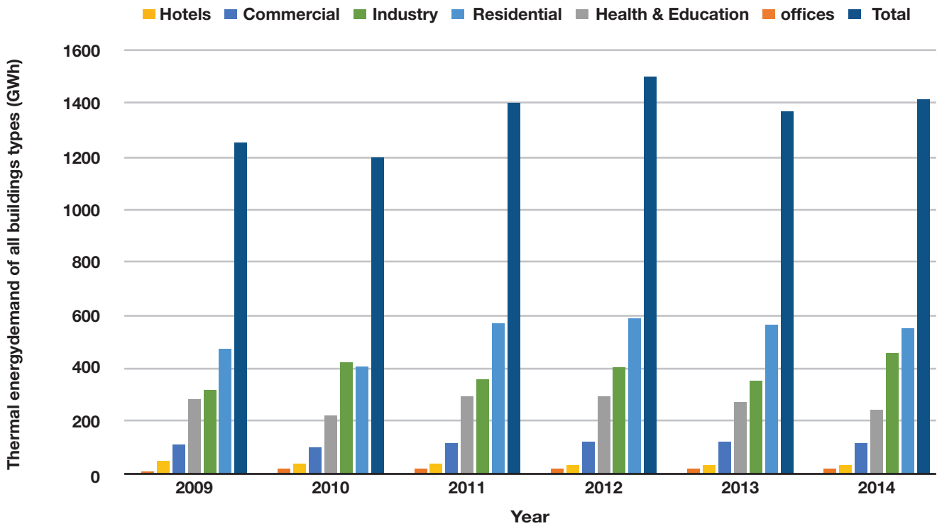
Figure 25: Thermal energy demand (GWh) of the building sector 2009–2014
