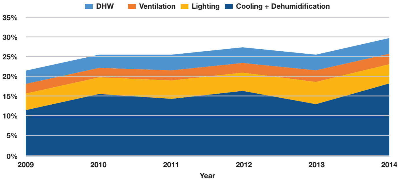
Residential sector usages as shares of the total Lebanese electricity demand
