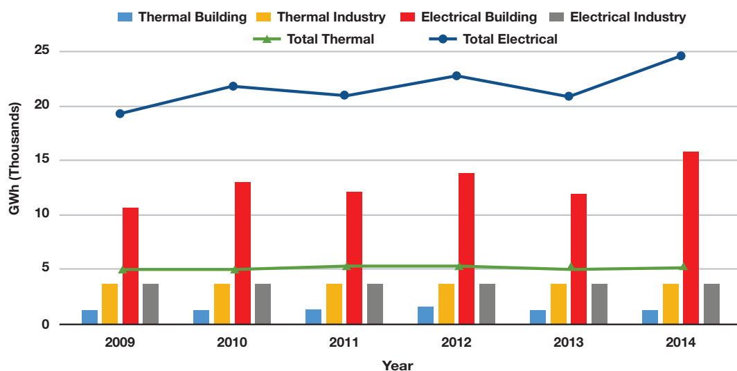
Thermal and electrical energy in the building and industrial sectors 2009–2014
