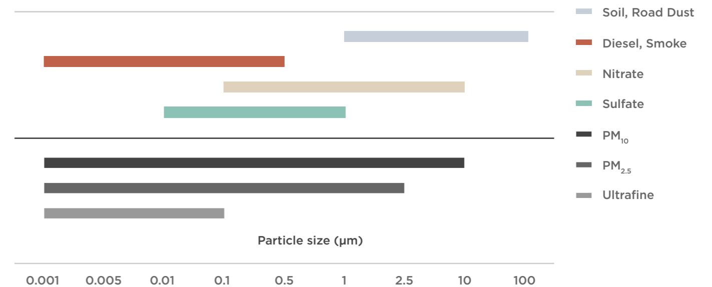
Figure 1. A: Graphic representation on a logarithmic scale showing example sources of different sized air pollution particles (blue, red, yellow, green) and the size fractions of particulate matter to which they contribute (dark to light grey) 13 .
