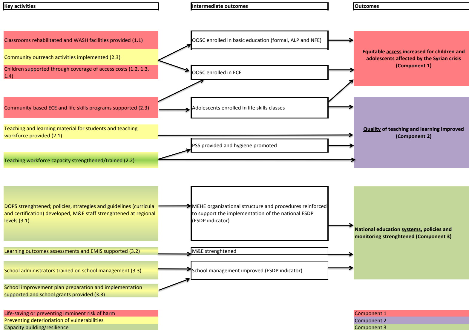
Figure 3: Log frame
